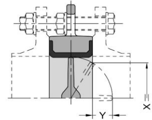
IN LINE INSTALLATION
