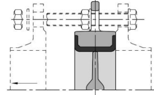
DEAD END SERVICE (6 bar MAX.)
