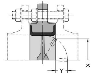
IN LINE INSTALLATION
