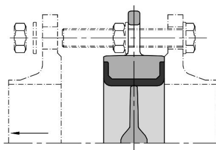
DEAD END SERVICE
